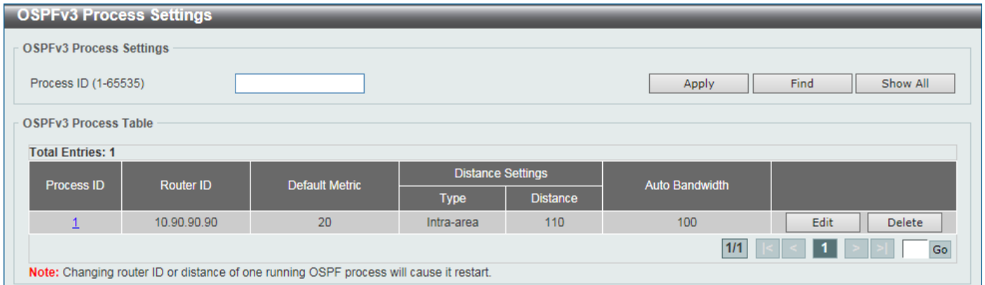
Figure 6-78 OSPFv3 Process Settings Window
