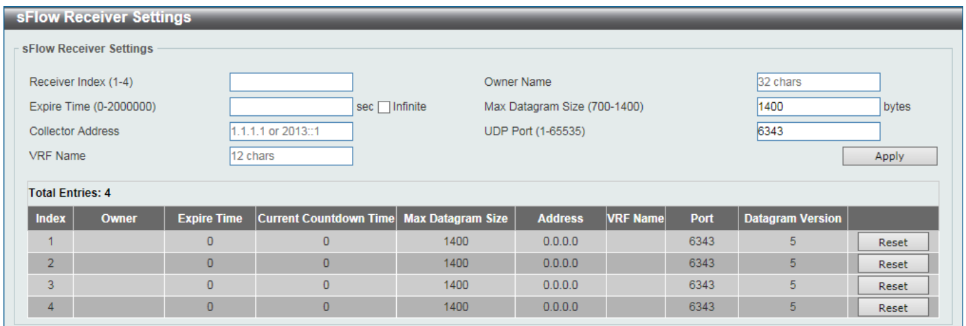
Figure 13-19 sFlow Receiver Settings Window
