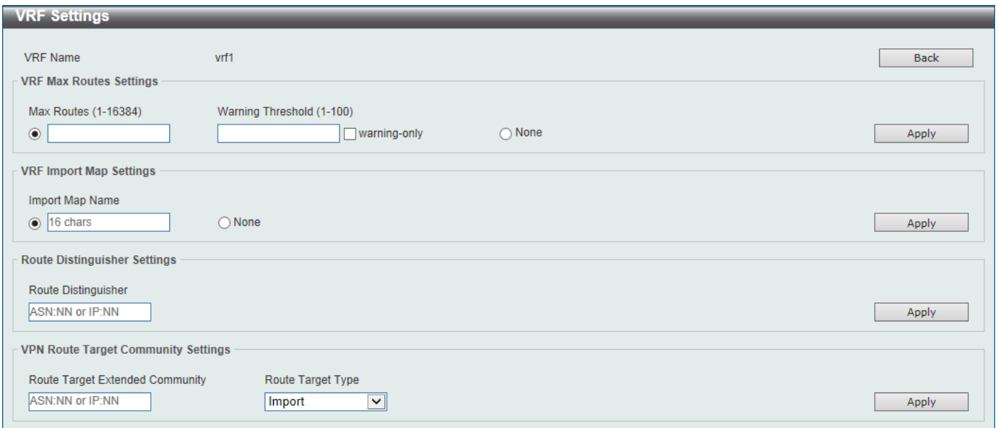
Figure 6-35 VRF Settings (Edit) Window
