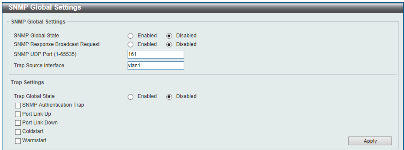
Figure 4-7 SNMP Global Settings Window
