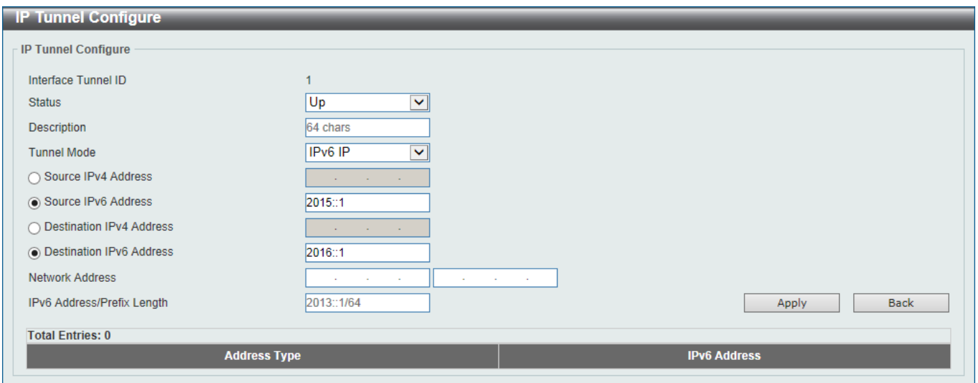
Figure 6-32 IP Tunnel Settings (Edit) Window
