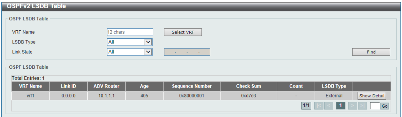
Figure 6-70 OSPFv2 LSDB Table Window
