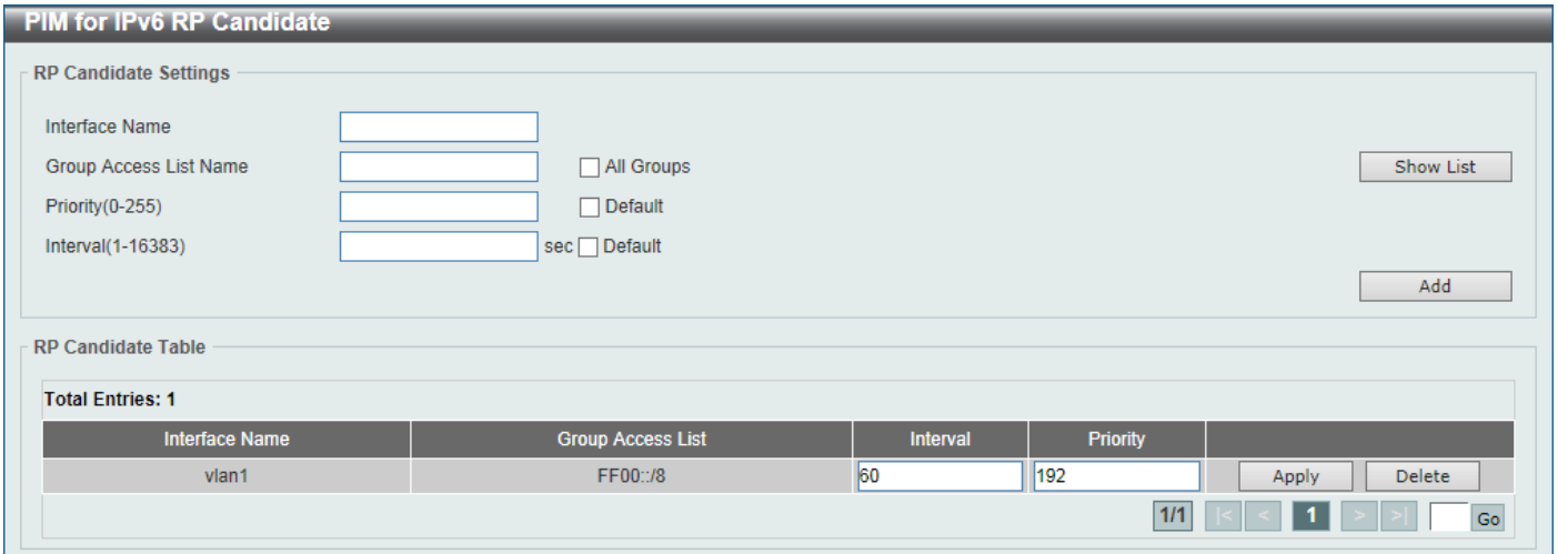
Figure 6-138 PIM for IPv6 RP Candidate (Edit) Window
