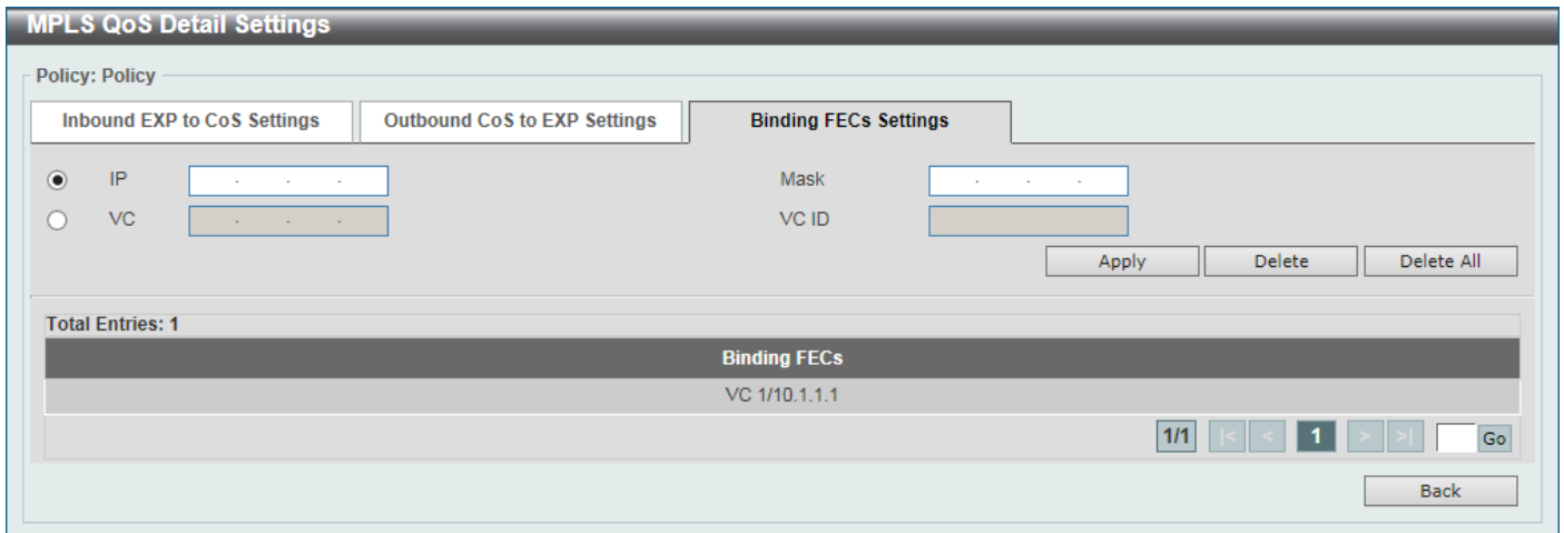
Figure 11-22 MPLS QoS Settings (Edit, Binding FECs Settings) Window
