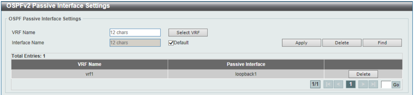
Figure 6-56 OSPFv2 Passive Interface Settings Window
