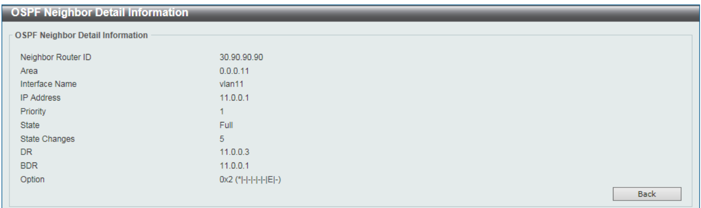
Figure 6-75 OSPFv2 Neighbor Table (Show Detail) Window
