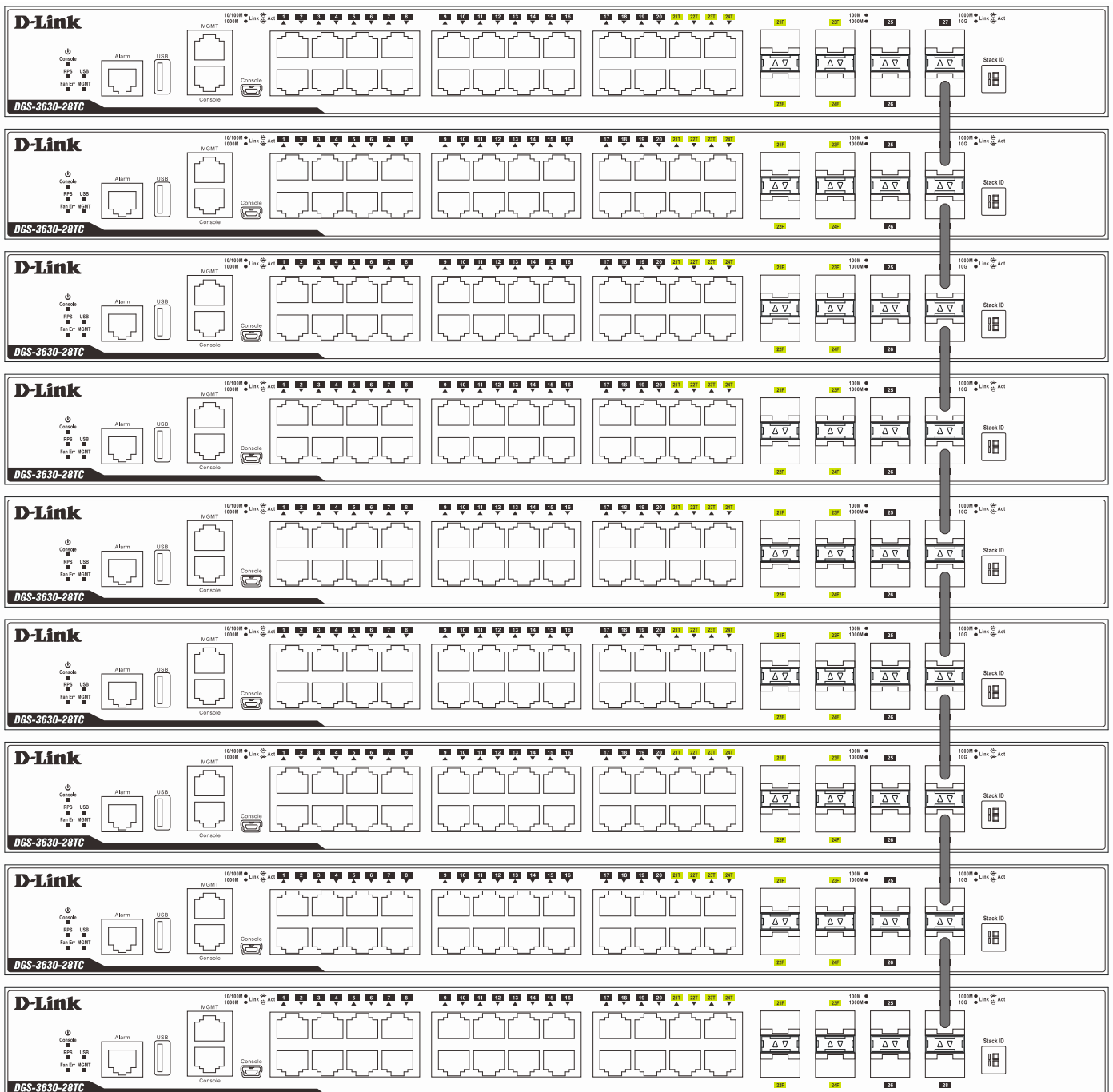
Figure 4-82 Duplex Chain stacking topology (SFP+)
