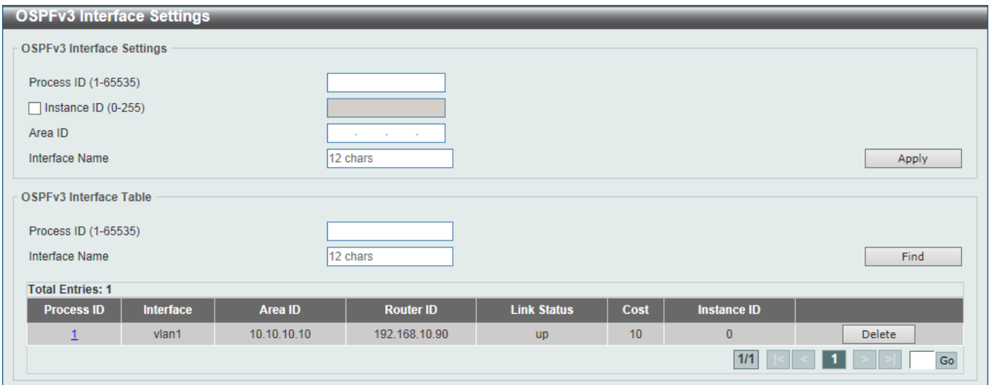
Figure 6-85 OSPFv3 Interface Settings Window
