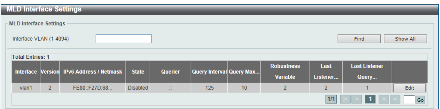
Figure 6-101 MLD Interface Settings Window
