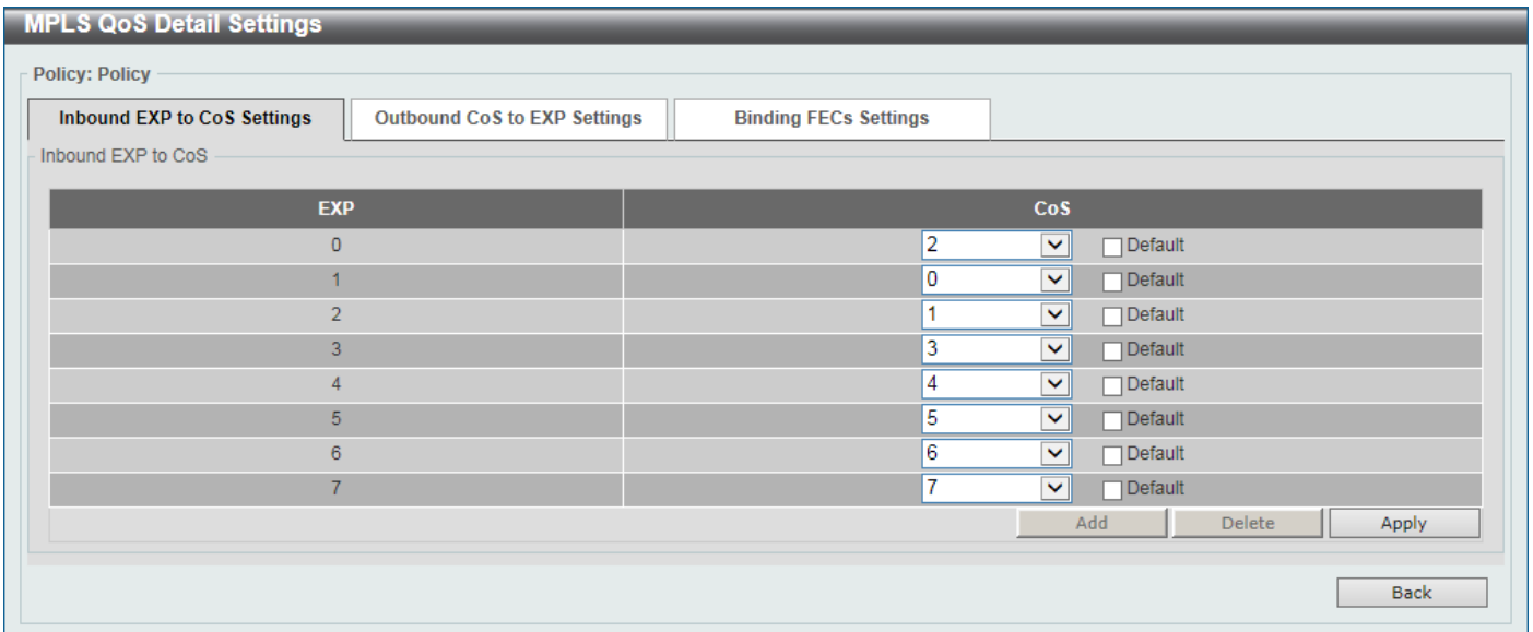
Figure 11-19 MPLS QoS Settings (Edit, Add) Window
