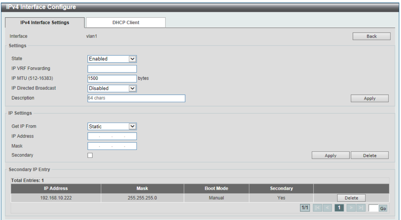
Figure 6-9 IPv4 Interface (Edit) Window
